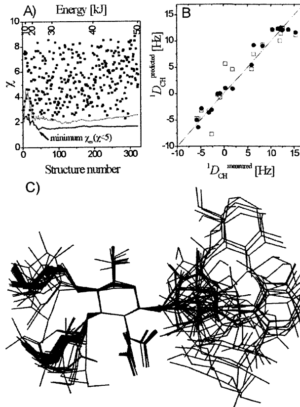
Figure 2. (A) \chi values for predictions of ^1D_{CH} in LNF-2 made by TRAMITE for individual structures ( \bullet ), using \langle \cos^2\theta_{ii} \rangle for the structures 1 to j (with j varying from 1 to the total of structures) (gray line), and filtering the structures with \chi_{\text{indiv.}} > 5 (black line). (B) Correlations for model 81 ( \square ) and for the filtered average structures where \chi was minimum ( \bullet ). (C) Superimposition of the 24 structures on the central GlcNAc residue that, averaged, best reproduce the ^1D_{CH} values.
